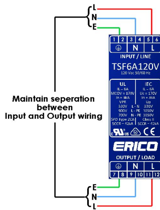
Figure 1: Wiring Diagram
